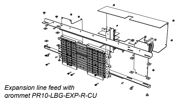
Expansion line feed PR10-LBx-x
