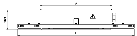
Expansion line feed PR10-LBx-x
