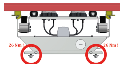
After alignment, fasten the M8 bolts in the PCT-MB (please follow mounting instructions for torque)
