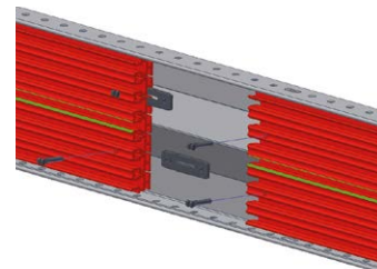
Connecting housing PR7 with set PR7-J
