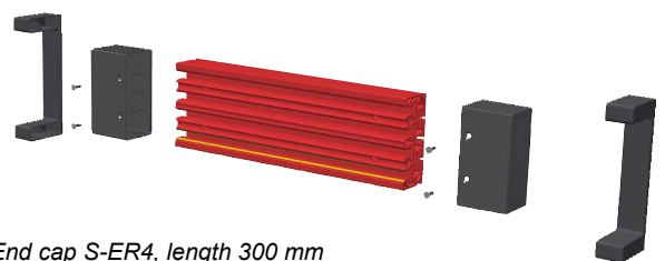
Set End cap S-ER4, length 300 mm
