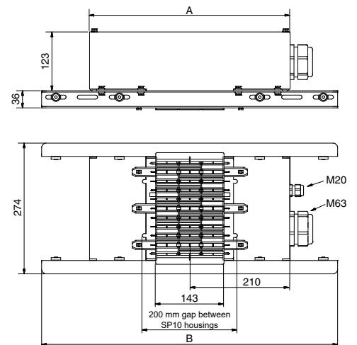
Line feed PR10-LB63/20
