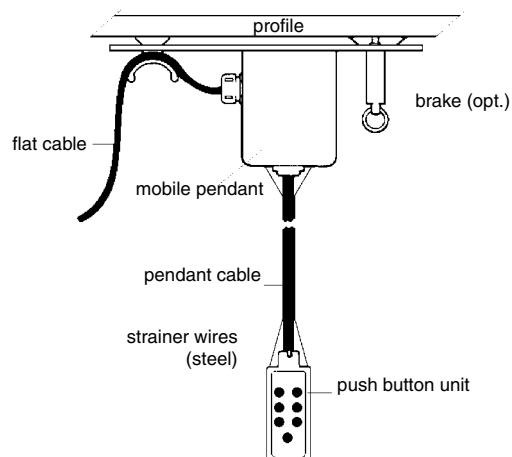
Mounting diagram
