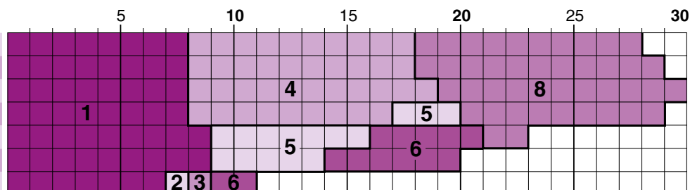
Winding length Lw (m), Case 1 h \leq 1 m
